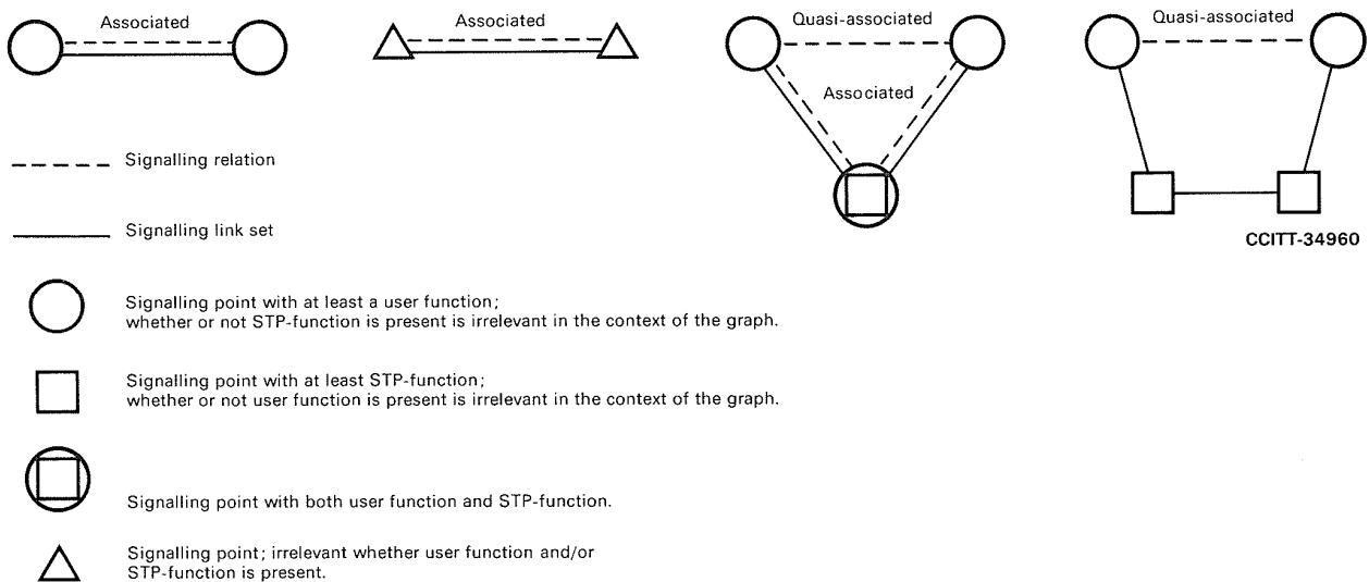
FIGURE 1/Q.700 Examples of associated and quasi-associated signalling modes and definition of signalling network graph symbols
