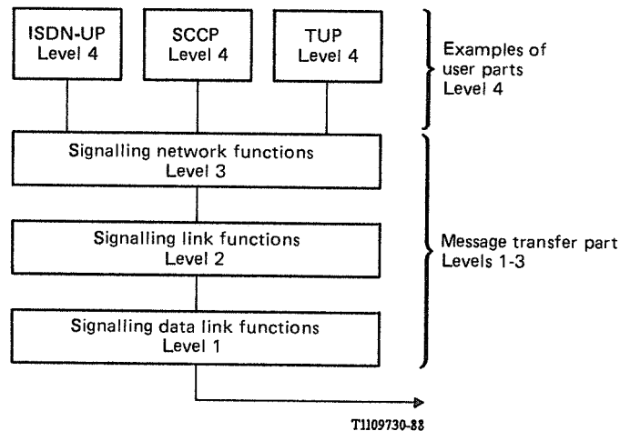
FIGURE 3/Q.700 CCITT No.7 functional levels
