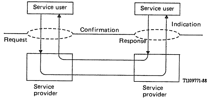
FIGURE 7/Q.700 Types of service primitives
