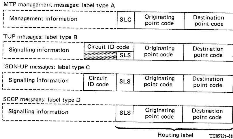
Figure 10/Q.700 CCITT SS No. 7 message label types
