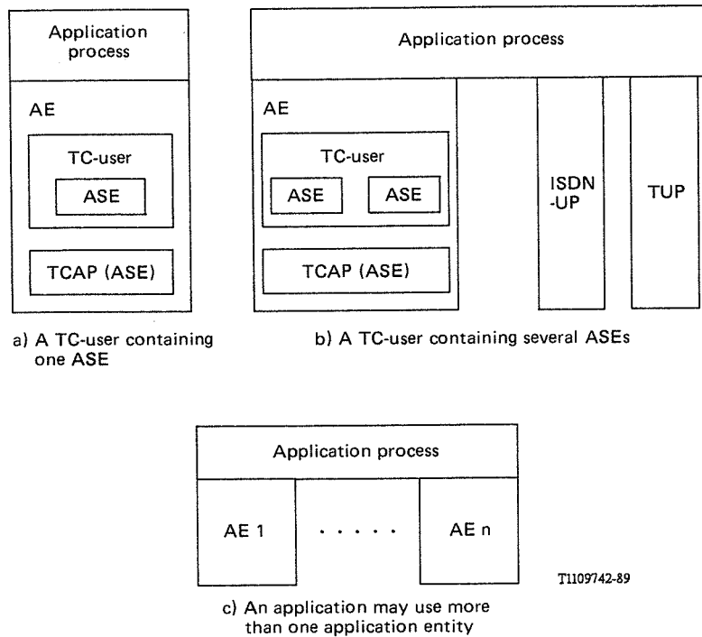
FIGURE 4/Q.700 Example of the relationship between the application process, AEs and ASEs
