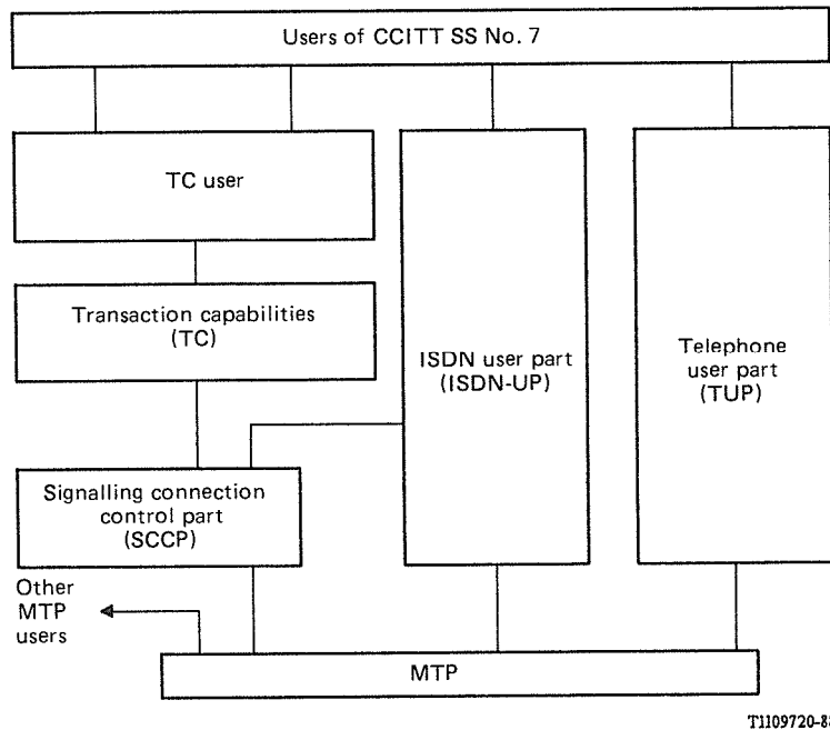
FIGURE 2/Q.700 Architecture of CCITT SS No. 7
