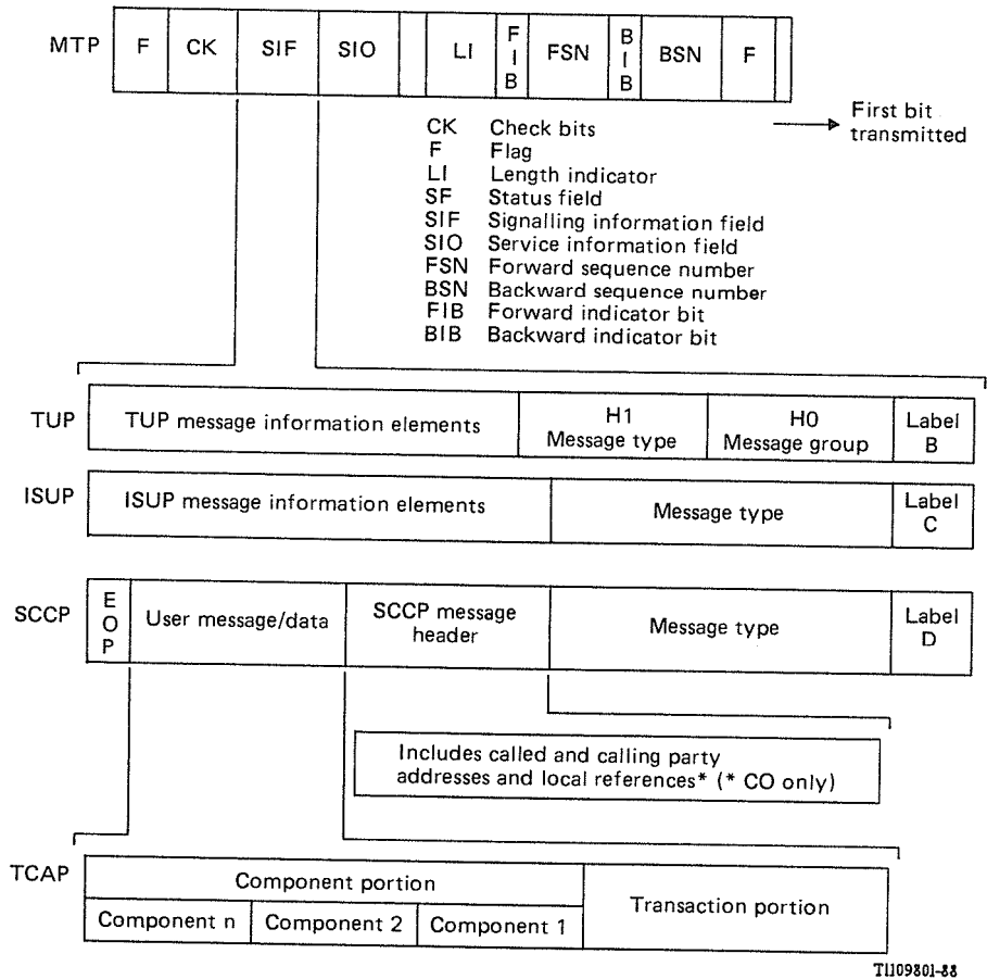
Figure 11/Q.700 CCITT No. 7 signalling message structure
