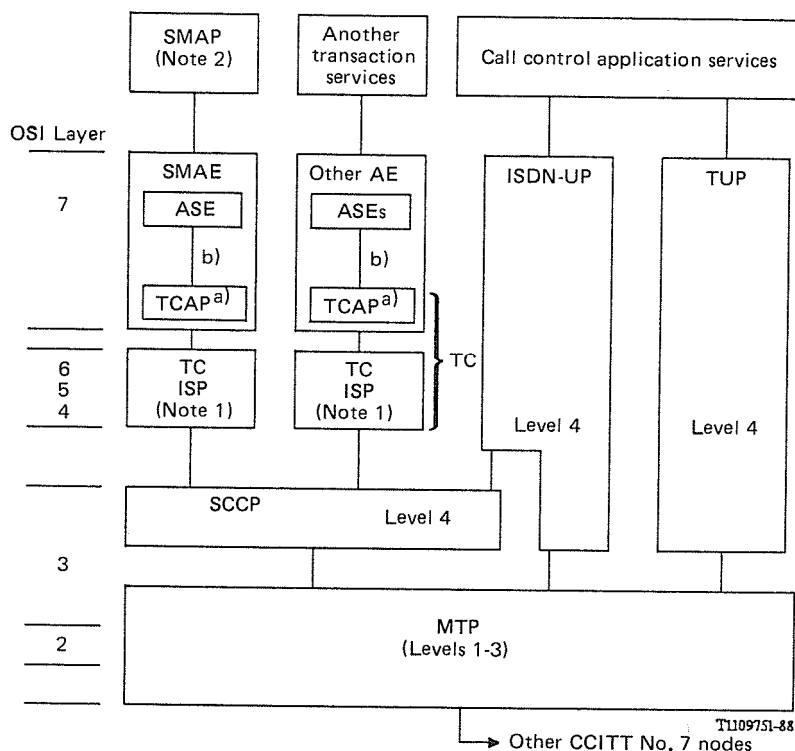
Figure 5/Q.700 shows the relationship between SCCP, TC, and ASEs to the OSI 7 Layer Reference Model.
