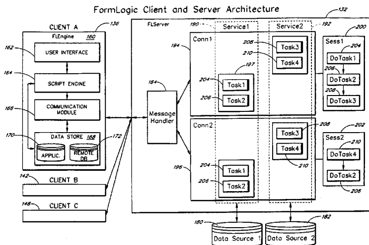
FormLogic Client and Server Architecture
