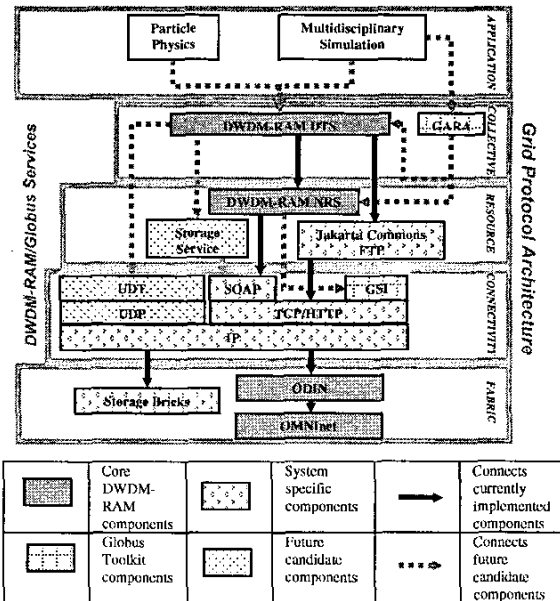
Figure 2: The DWDM-RAM architecture
