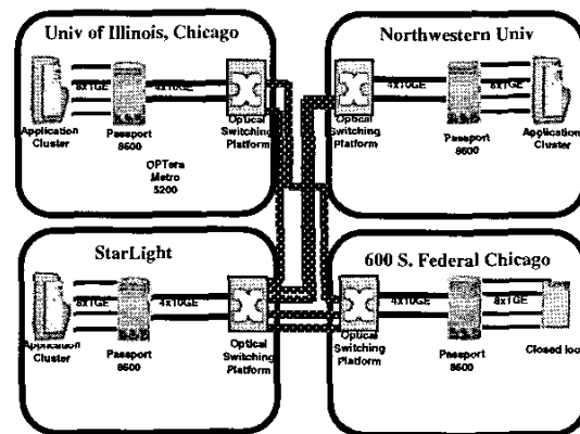
Figure 3: OMNInet core nodes
