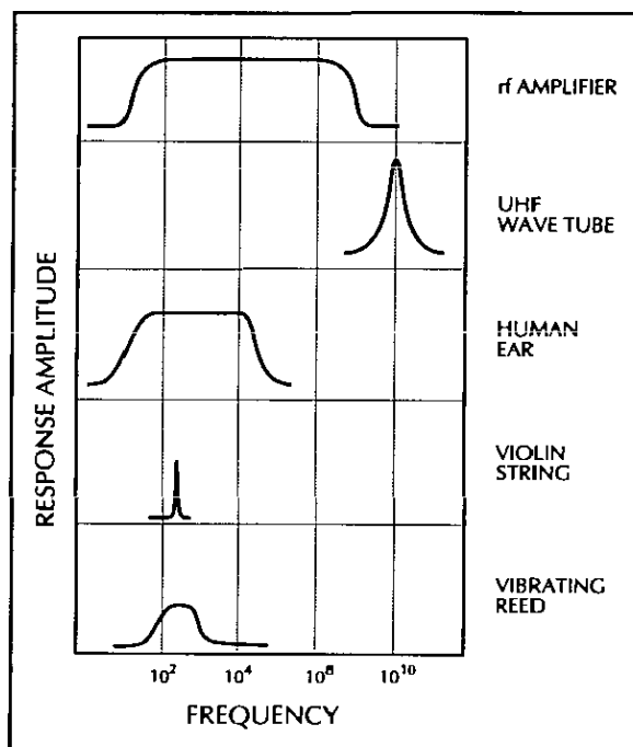
representative frequency response of various devices
